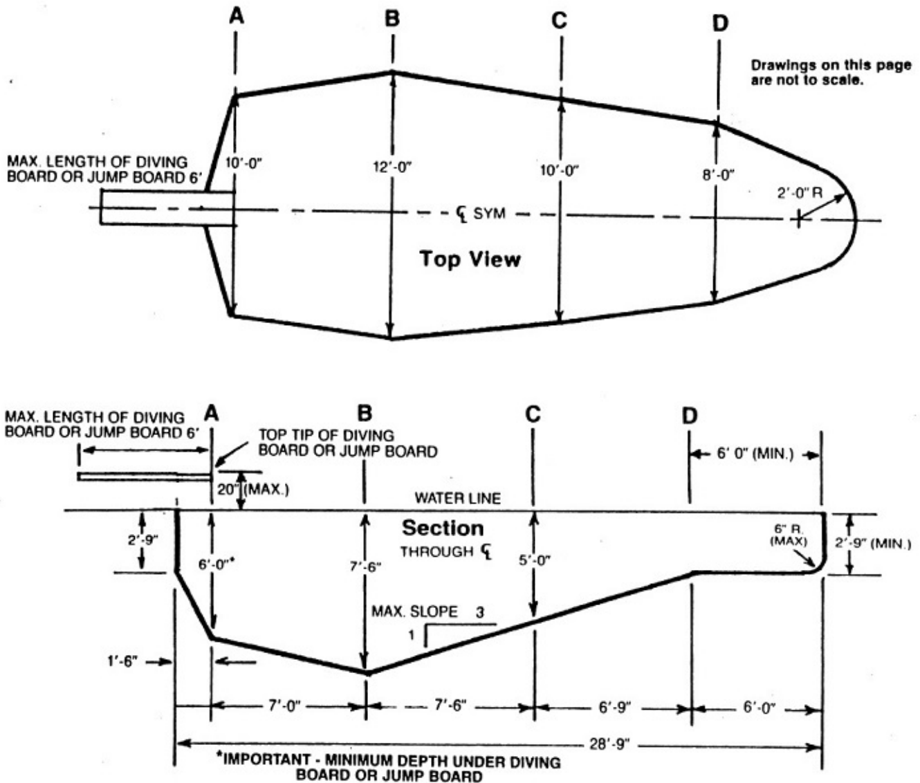
FIGURE R326.10(5) MINIMUM DIMENSIONS FOR A TYPE I POOL
