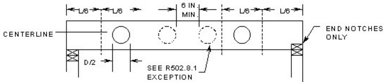
SOLID LUMBER JOISTS 2 X 8 AND LARGER
